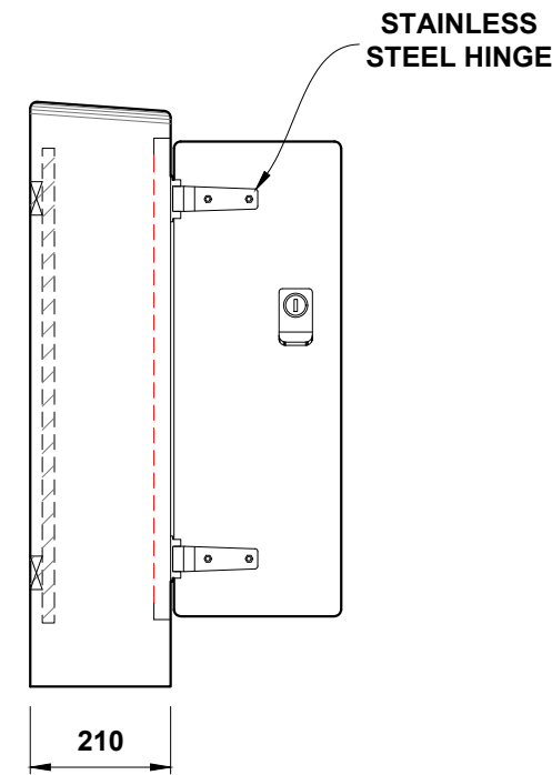
Elevation (C) (l/h side) Door Open
